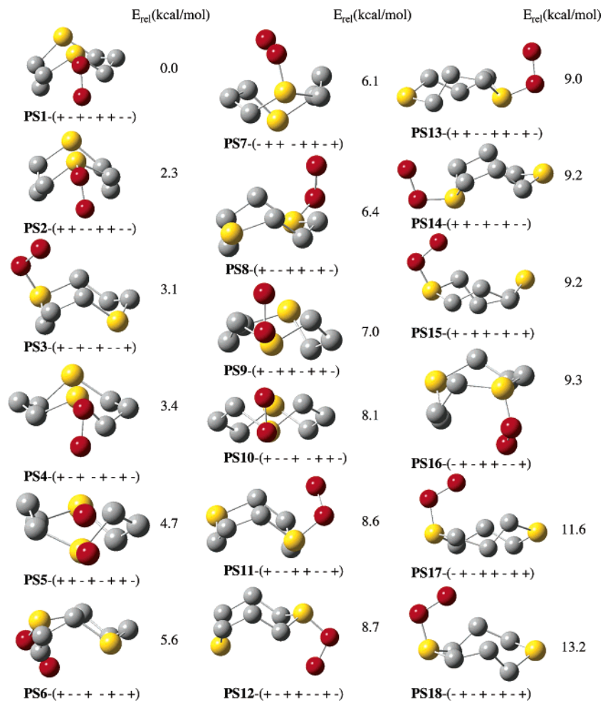
Figure 3. Conformational minima for 1,5-dithiacyclooctane persulfoxides and their relative energies with hydrogens removed for clarity.
