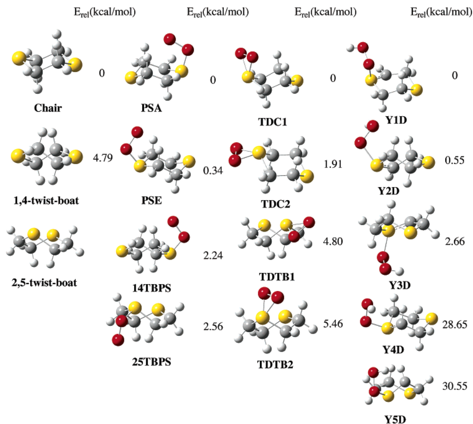
Figure 2. Conformations of 1,4-dithiane and its persulfoxides, thiadioxiranes, and hydroperoxy sulfonium ylides.
