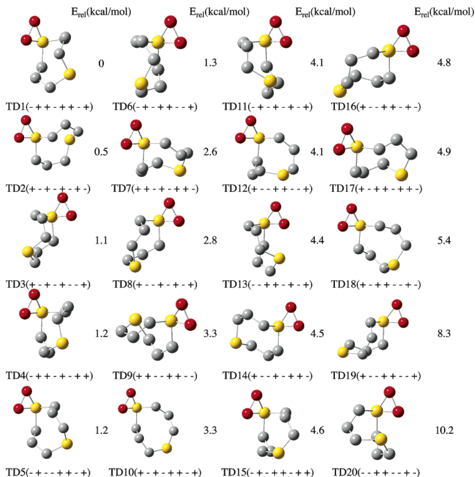
Figure 4. 1,5-Dithiacyclooctane thiodioxiranes with the hydrogens removed for clarity.
