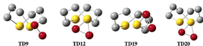
Figure 5. Unusual twist-boat–twist-boat thiodioxiranes with hydrogens removed for clarity.
